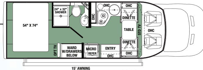
15' AWNING TS2381 (Ford EcoBoost 3.5L gas engine)
