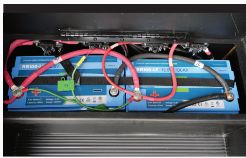
Dual Low-Temp Lithium Auxiliary Batteries (200aH Total) With a built-in heater, these batteries can charge at temperatures as low as -20°C.
